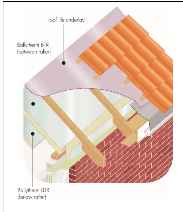
Figure 1 Ballytherm BTR Pitched Roof Insulation
